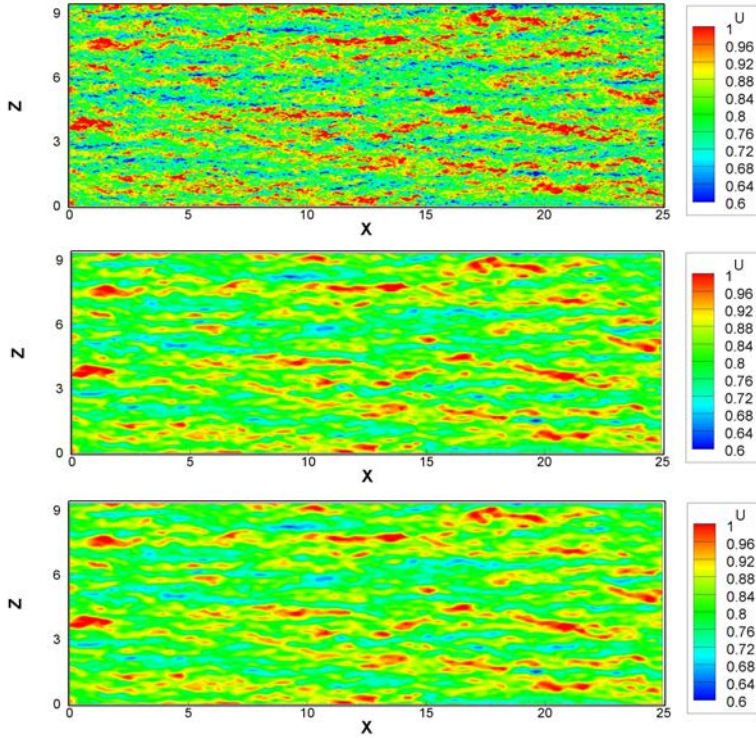
Figure 6: Contour plots of u at y = \Delta_y (taking y = 0 to be the wall) for the unfiltered DNS, Gaussian filtered, and tophat filtered fields. The horizontal filtering is done at \Delta x^+ = 192 (or \Delta_x \approx 2\Delta_y ), \Delta_z^+ = 97 (or \Delta_z \approx \Delta_y ). The resolution of original DNS is \Delta x^+ = 12 , \Delta_z^+ = 6 .
